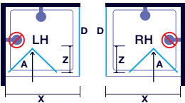
Hinged Bifold Door with Side Panel
