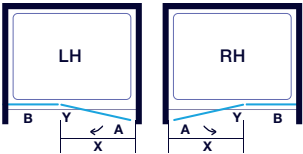
Hinge and Inline Door a Recess
