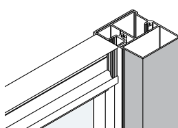
With cover strip - conceals all fixings
