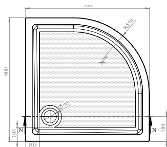
900 x 900 Anti-Slip Quadrant Tray - RSQG90
