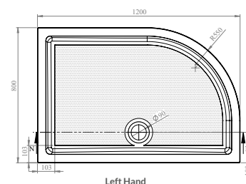
1200 x 800 Anti-Slip Quadrant Tray - Left Hand - RSQG128L
