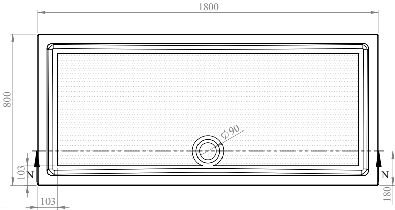
1800 x 800 Anti-Slip Tray - RSTG188
