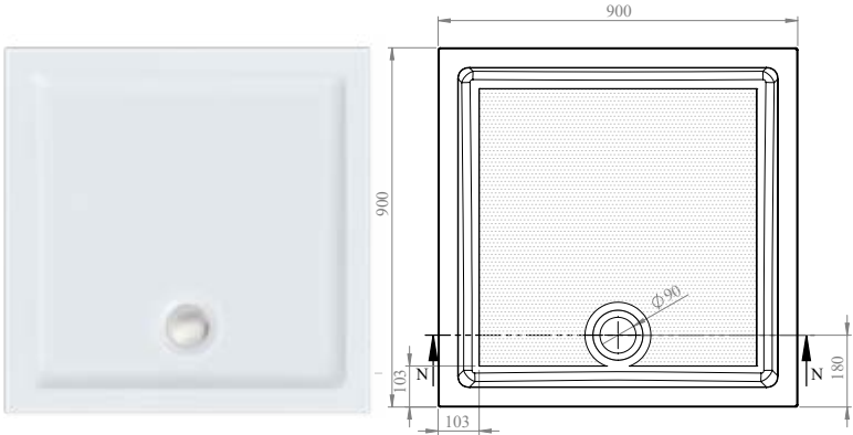
900 x 900 Anti-Slip Tray - RSTG90
